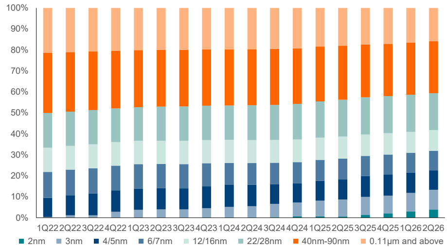
Figure 7: Capacity breakdown
